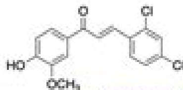
compound C4
