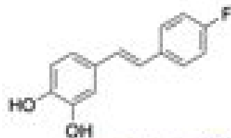
compound ST3
