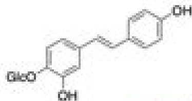
polydatin
