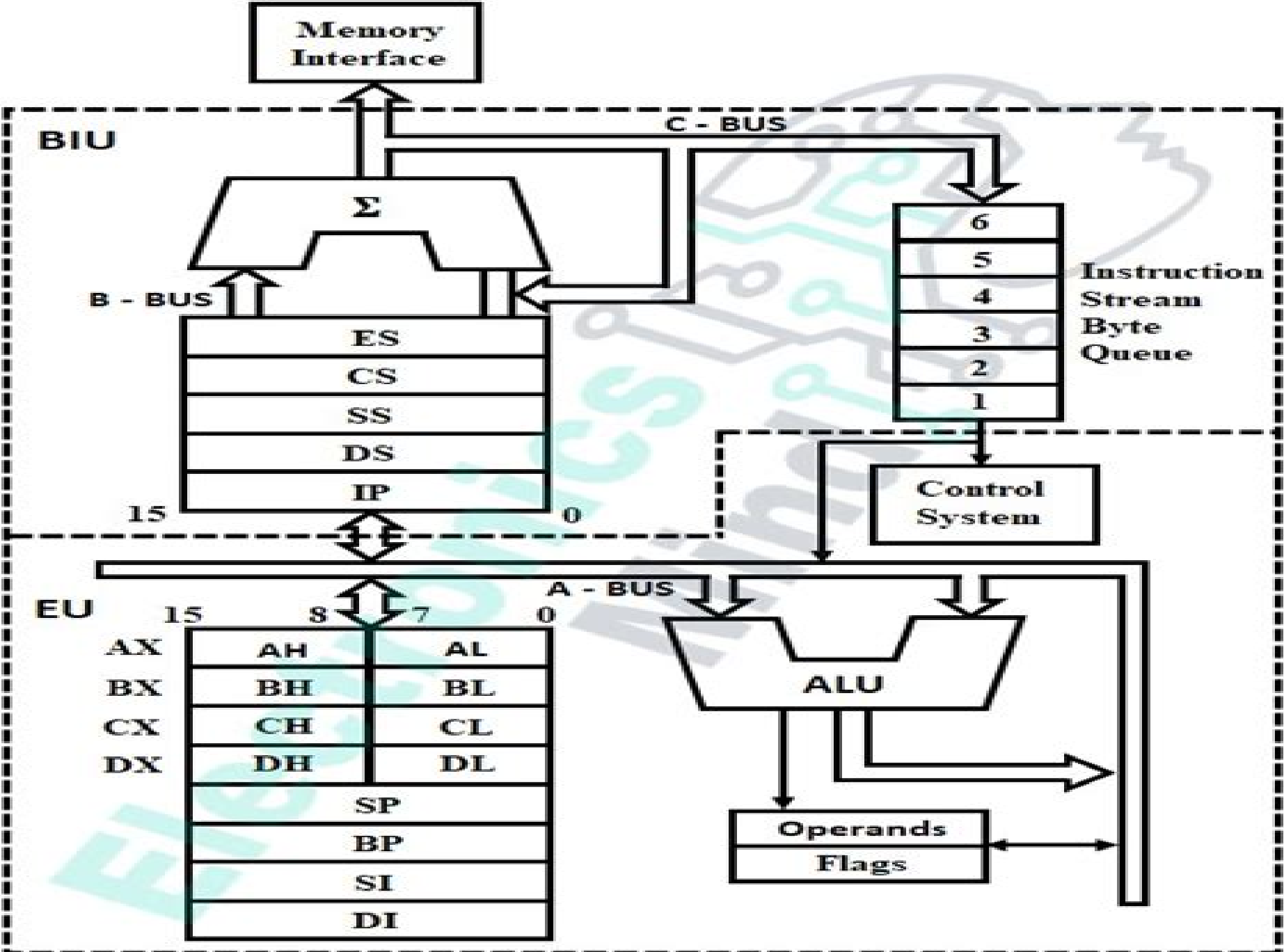
8086 Internal Architecture
