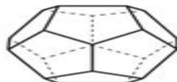
dodecahedron
