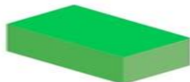
cuboid
