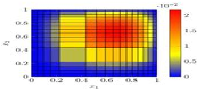
(a) Solution on r -adaptive mesh.
