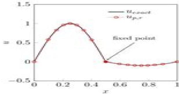
(a) Solution on r -adaptive mesh.
