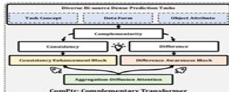
Fig. 1: Visual outline of the proposed ComPtr. For diverse bi-source dense prediction tasks, our method is based on the generic concept of complementarity. The consistency enhancement block (Sec. 3.2.3) and difference awareness block (Sec. 3.2.4) are constructed based on the proposed efficient aggregation-diffusion attention (Sec. 3.2.1) from the perspectives of consistency and difference, respectively. Such a design as a whole serves the implementation of the task-generic architecture.
