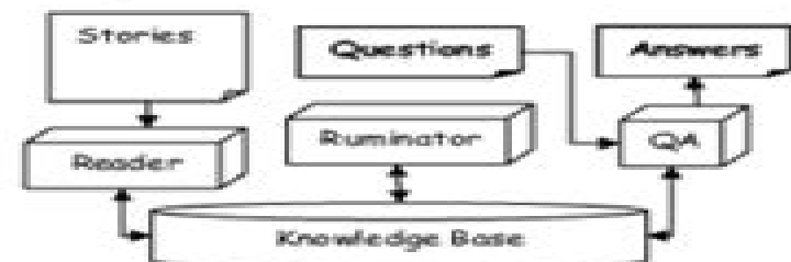
Figure 1: Learning Reader Architecture
