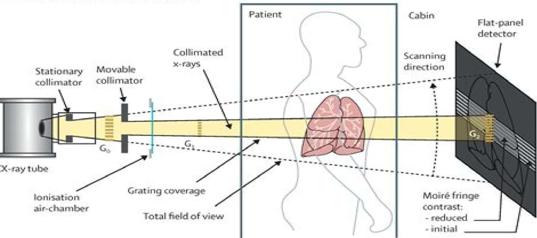
A X-ray dark-field demonstrator system
