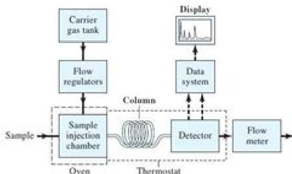
Figure 32-1 Block diagram of a typical gas chromatograph.
