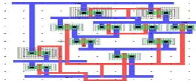
Figure 4: Layout of Gilbert cell multiplier
