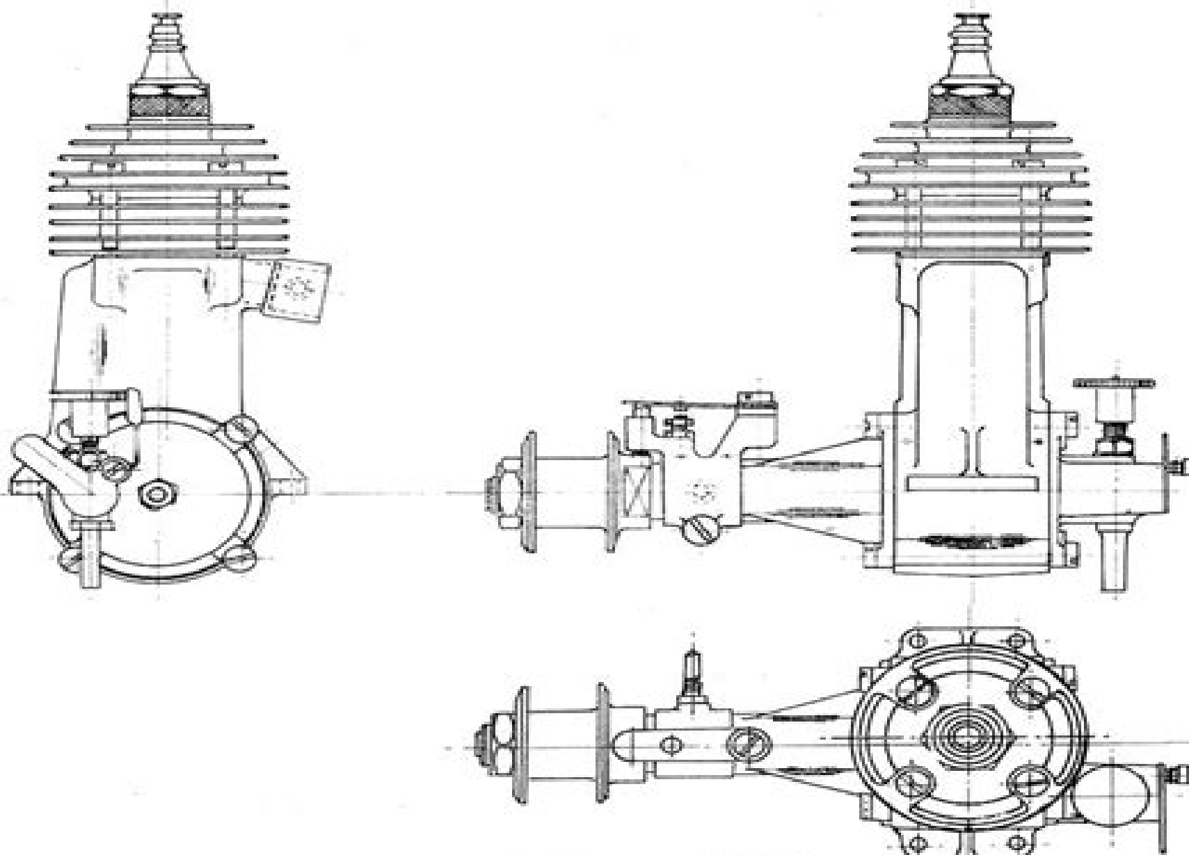
THE ATOM MINOR MK. III 6 cc. ENGINE 2\frac{3}{32} " BORE X \frac{7}{8} " STROKE
