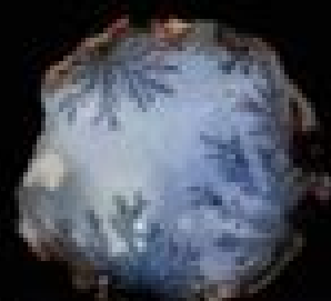
Dendritic Agate
