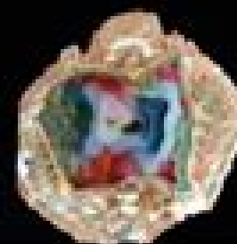
Thunder-egg Agate
