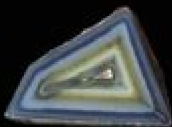
Polyhedroid Agate
