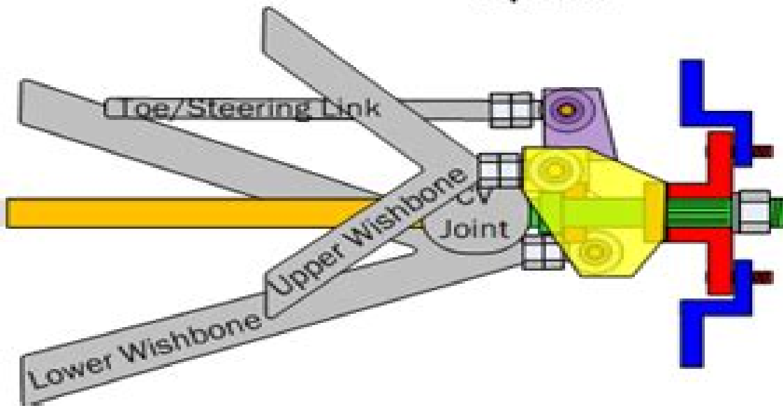
Top View
