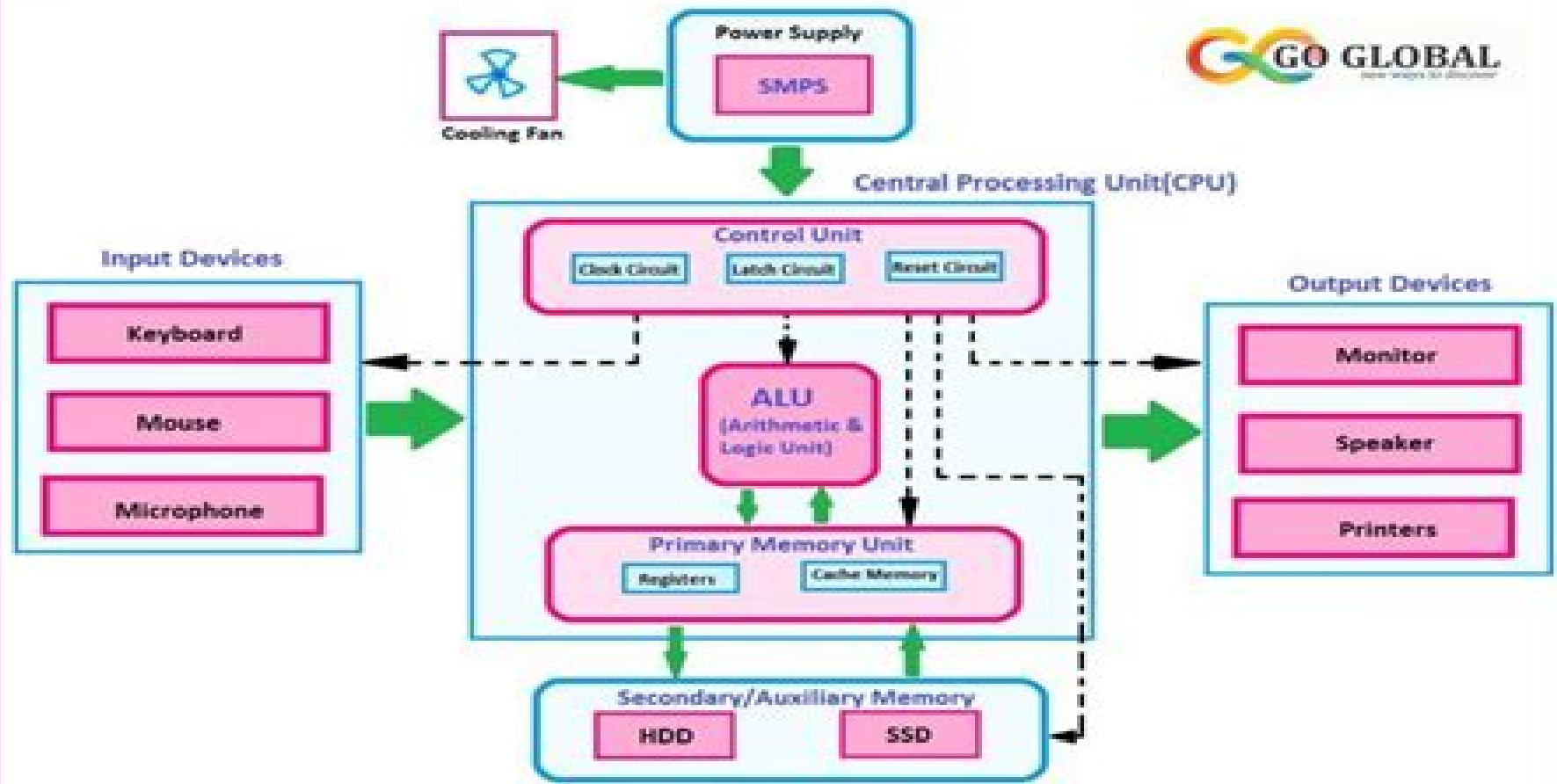
Computer Block Diagram
