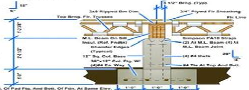
Figure 7-29 — Construction drawings.
