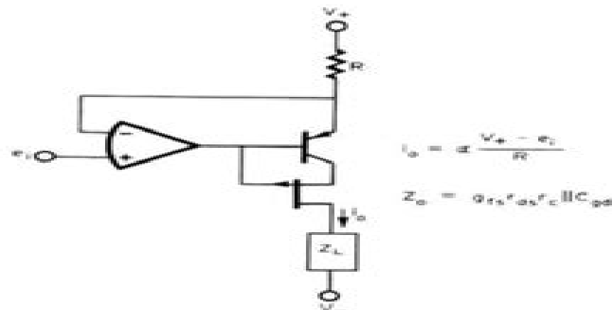
Fig. 3.13 An FET cascode bias greatly increases the output impedance of a bipolar transistor-controlled current source by essentially removing load voltage swing from the current source transistor.
