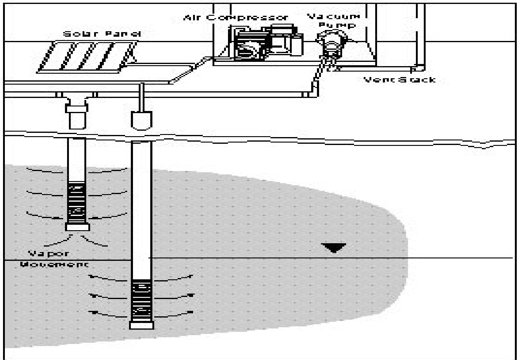
Subsurface Volatilization and Ventilation System (SVVS®)
