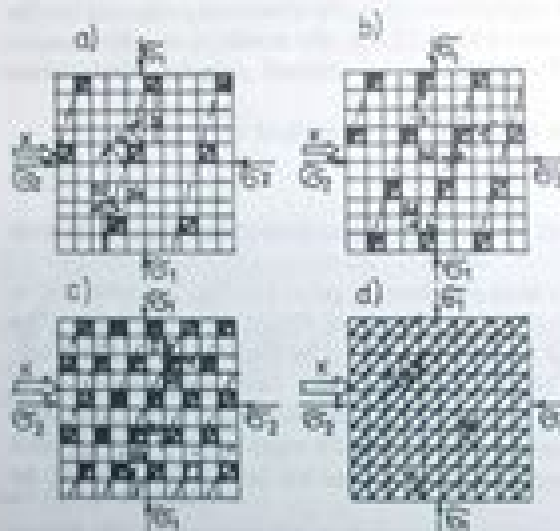
Fig. 2.6. Failure at micro-level according to Strohman. The small squares simulate mineral grains. The view is from of the arrow is as in the plot.
