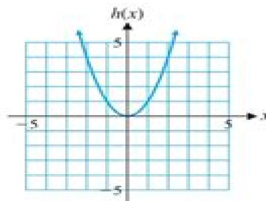
(B) Square function
