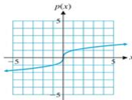
(E) Cube root function
