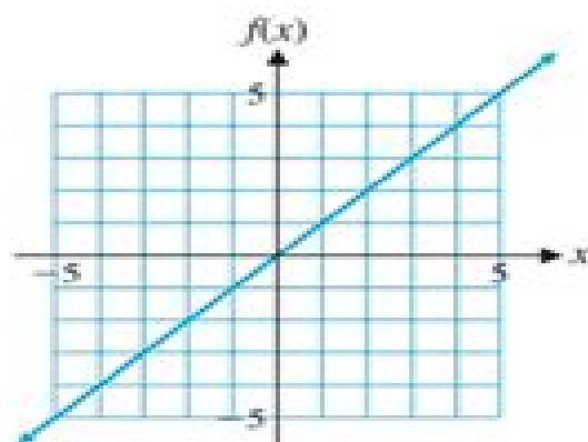
(A) Identity function
