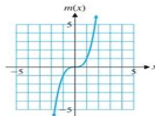
(C) Cube function
