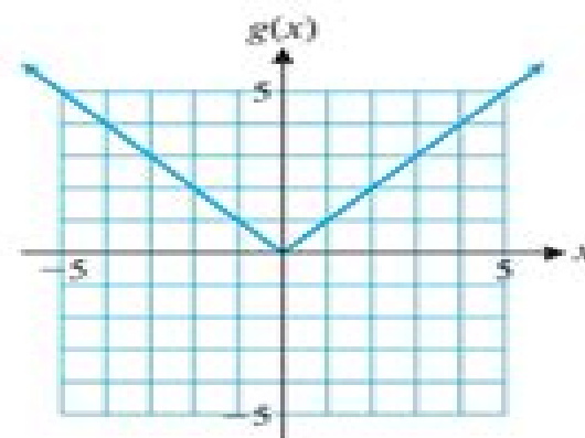
(F) Absolute value function
