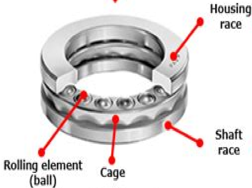
Thrust ball bearings
