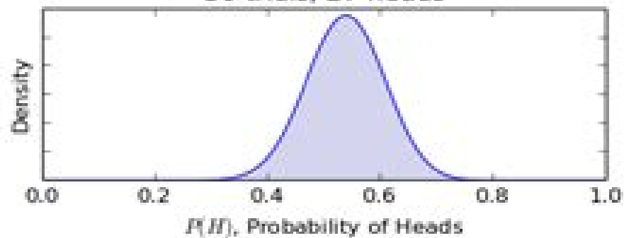
50 trials, 27 heads
