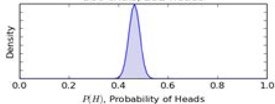
500 trials, 232 heads
