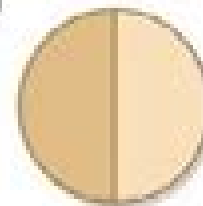
Fig. 4.2.14 of Stein and Wyssession, 2003
