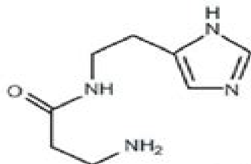
Carcinine
