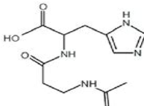
N-acetylcarnosine
