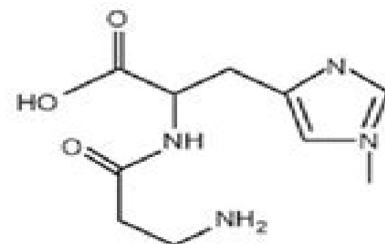
Balenine/Ophidine
