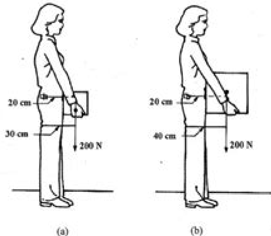
FIGURE 2.3. The influence of box size on the biomechanics of the back. The moment of the load in part (a) is M_0 = 0.3 \text{ m} \times 200 \text{ N} = 60 \text{ Nm} , while in part (b), M_0 = 0.4 \text{ m} \times 200 \text{ N} = 80 \text{ Nm} .
