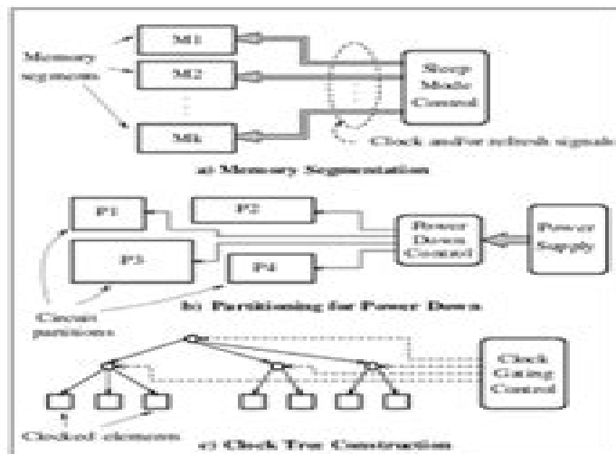
Figure 1: Circuit partitioning to exploit sleep mode
