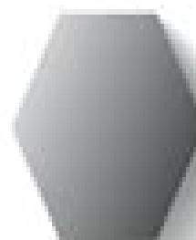
HEXAGONAL PRISM
