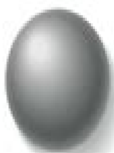
SPHERE
