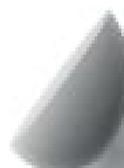
HALF-SPHERE
