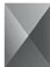
SQUARE PYRAMID
