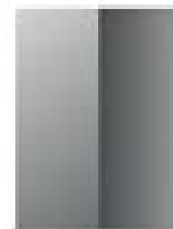
TRIANGULAR PRISM
