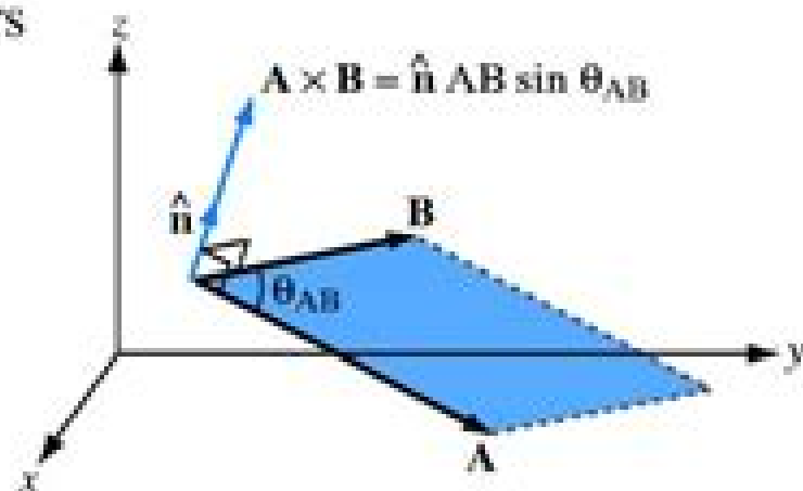
(a) Cross product
