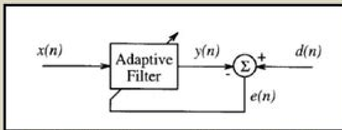
Simplified Block Diagram of the Adaptive filter
