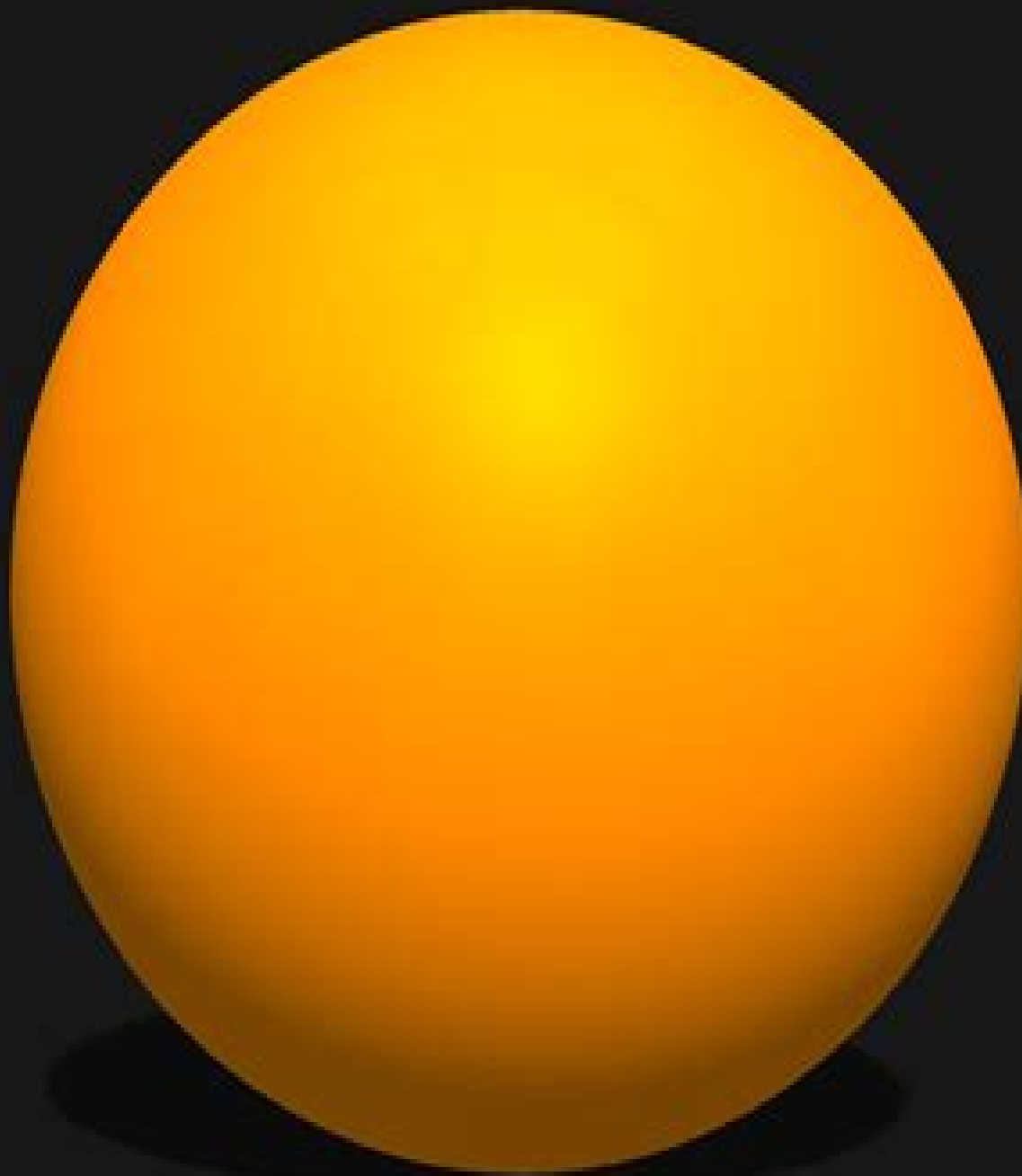
The Sun
