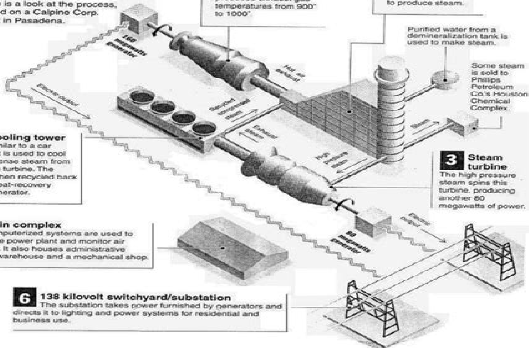
Figure I-1a. Cogeneration System Overview
