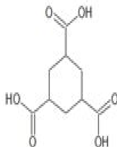
cyclohexane-1,3,5-tricarboxylic acid
