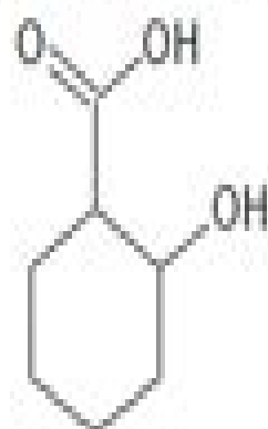
2-hydroxycyclohexanecarboxylic acid
