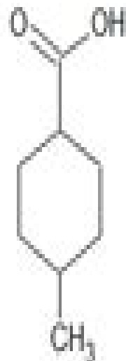
4-methylcyclohexanecarboxylic acid
