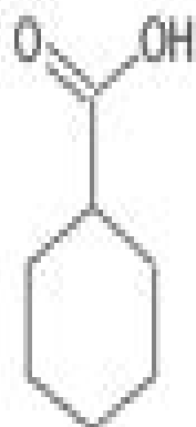
cyclohexanecarboxylic acid
