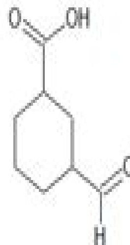
3-formylcyclohexanecarboxylic acid
