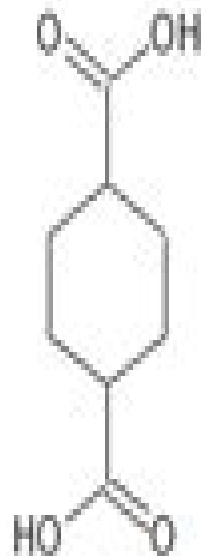
cyclohexane-1,4-dicarboxylic acid
