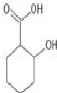
2-hydroxycyclohexanecarboxylic acid
