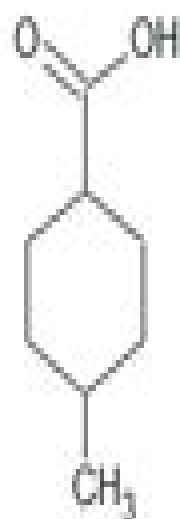
4-methylcyclohexanecarboxylic acid
