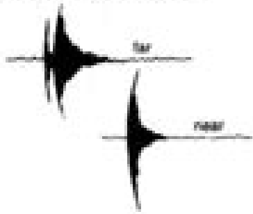
Short-period earthquakes
