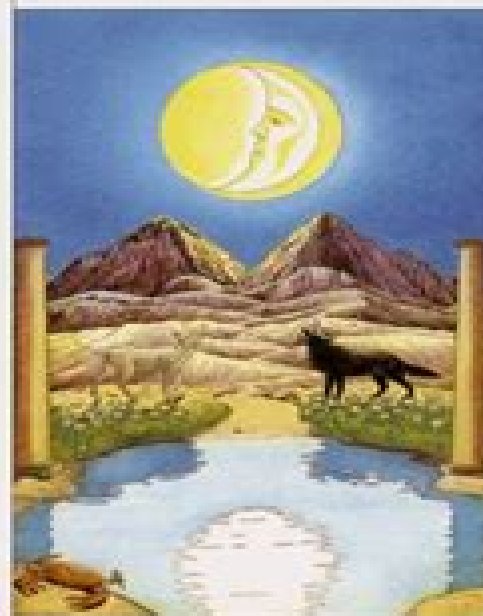
THE MOON
