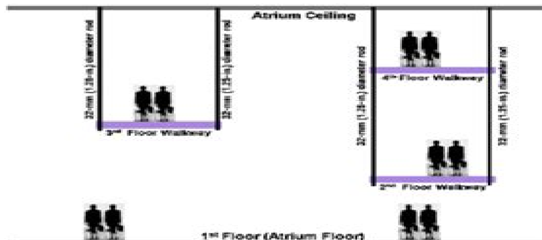
Fig. 1. Atrium of Hyatt Regency Hotel, Kansas City, Missouri
