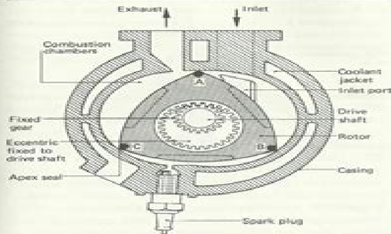
Figure 87 Spark ignition rotary engine
