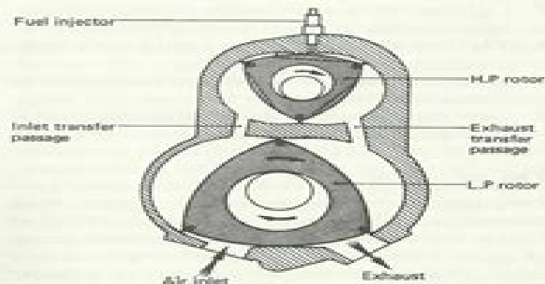
Figure 88 A two-stage rotary CI engine
