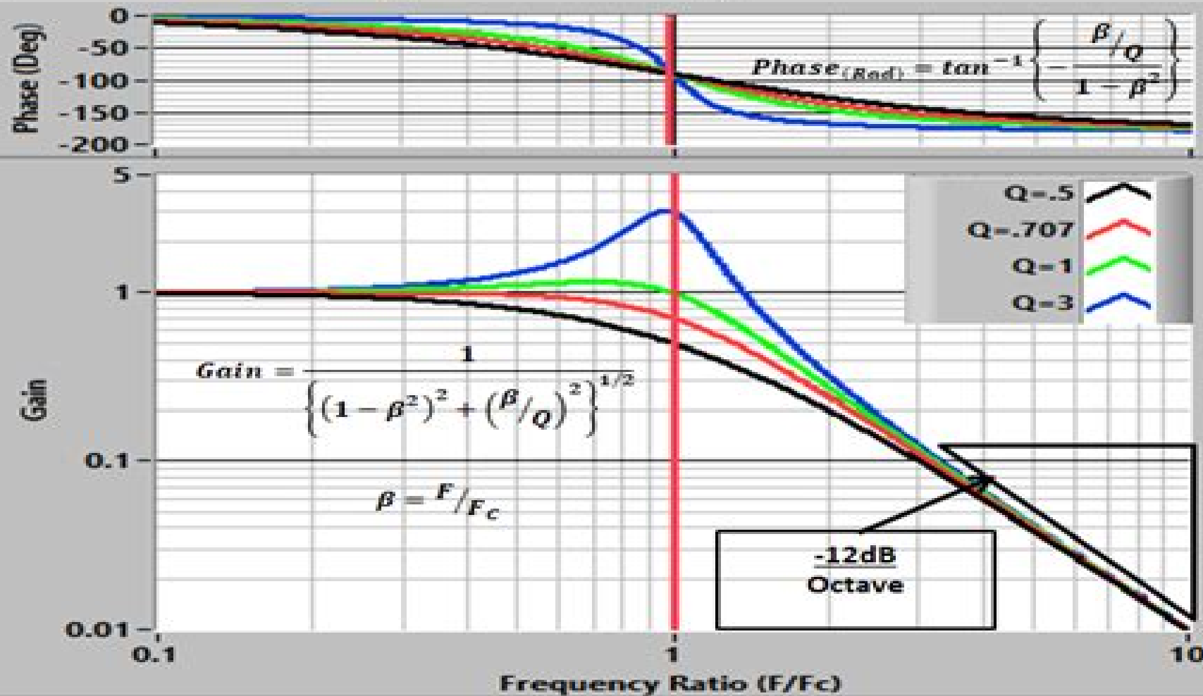
Figure 3: Two-Pole Low-Pass Filter: Q= 0.5, 0.707, 1.0, 3.0
