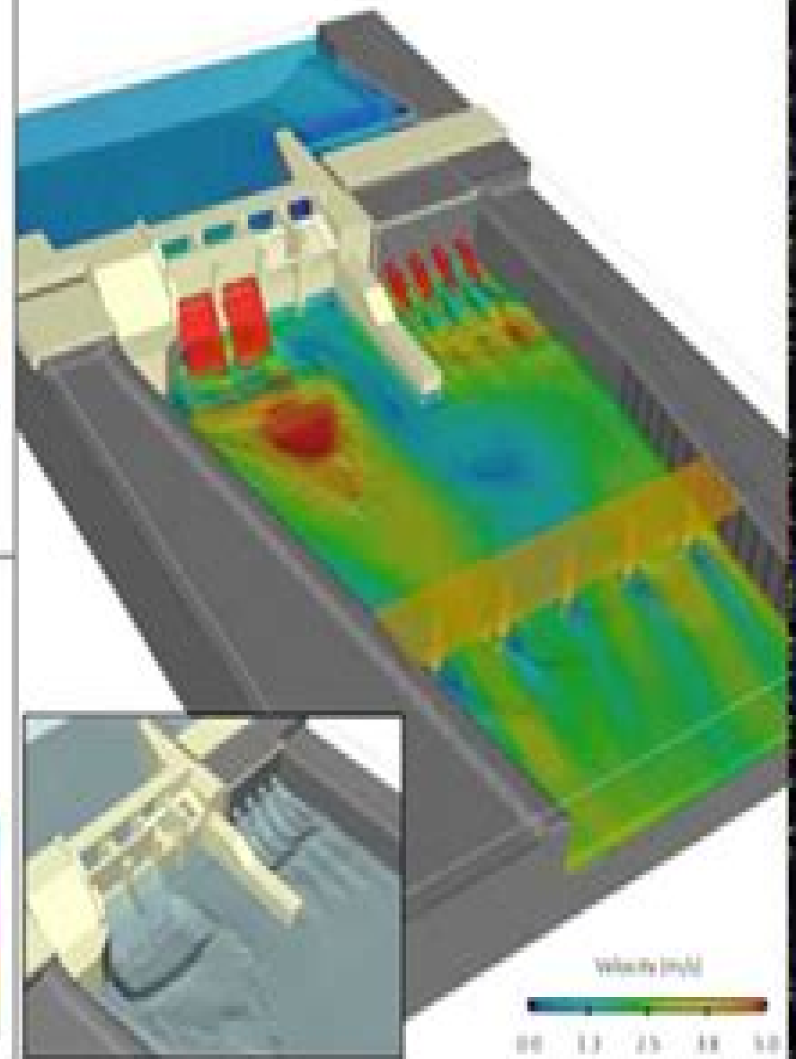
Velocity Field and Bed Height Changes
