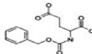
N-CBZ Lysine
