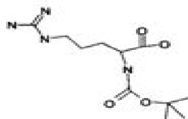
N-t-Boc Arginine
