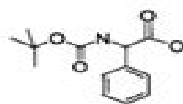
N-t-Boc Phenylglycine
