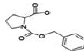
N-CBZ Proline
