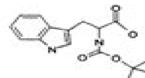
N-t-Boc Tryptophan
