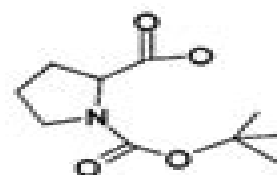
N-t-Boc Proline
