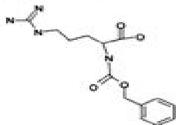
N-CBZ Arginine
