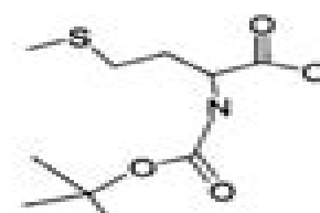
N-t-Boc Methionine
