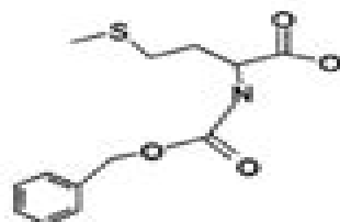
N-CBZ Methionine
