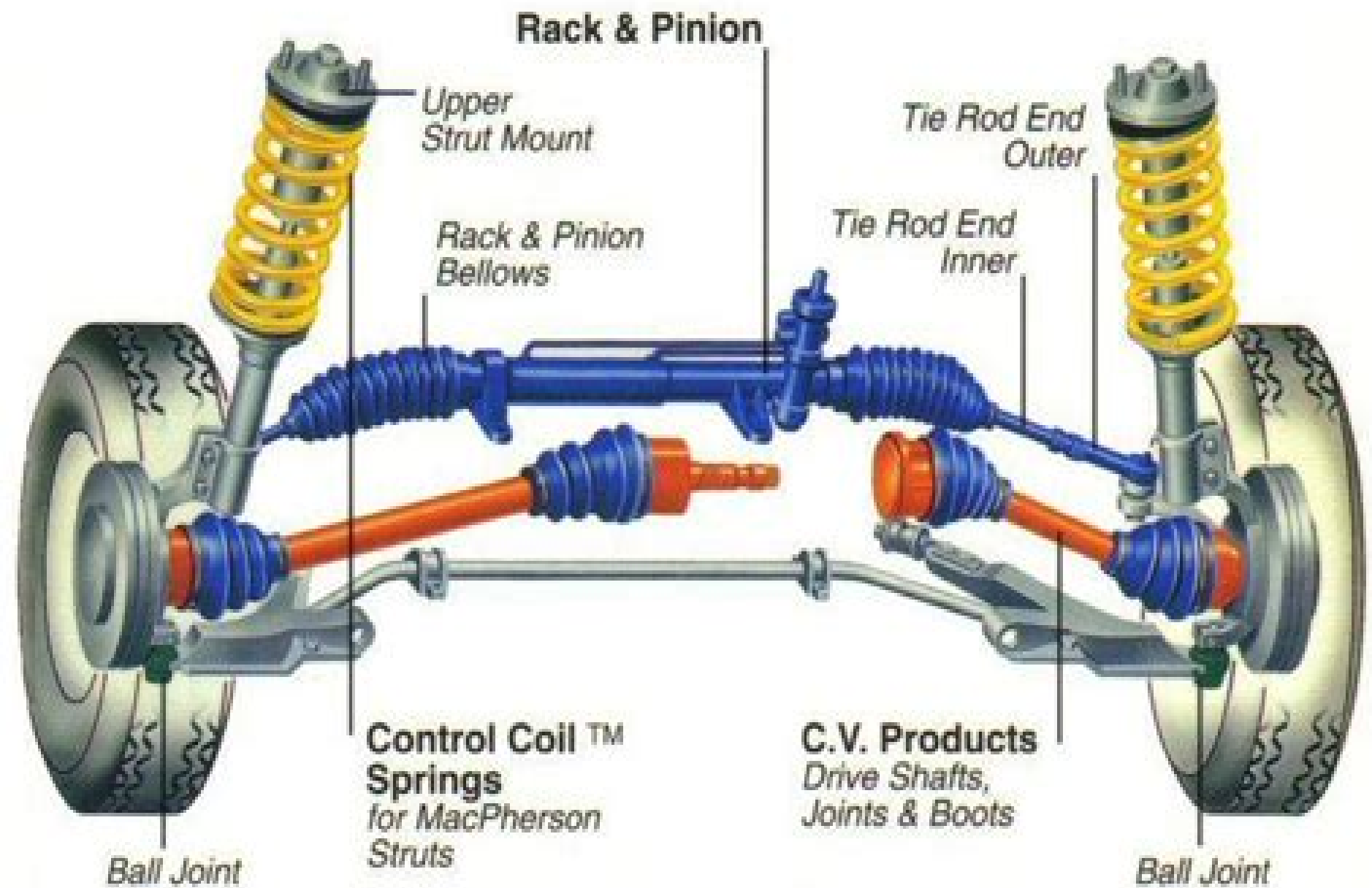
Front Wheel Drive Suspension
