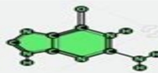
G - Guanine
